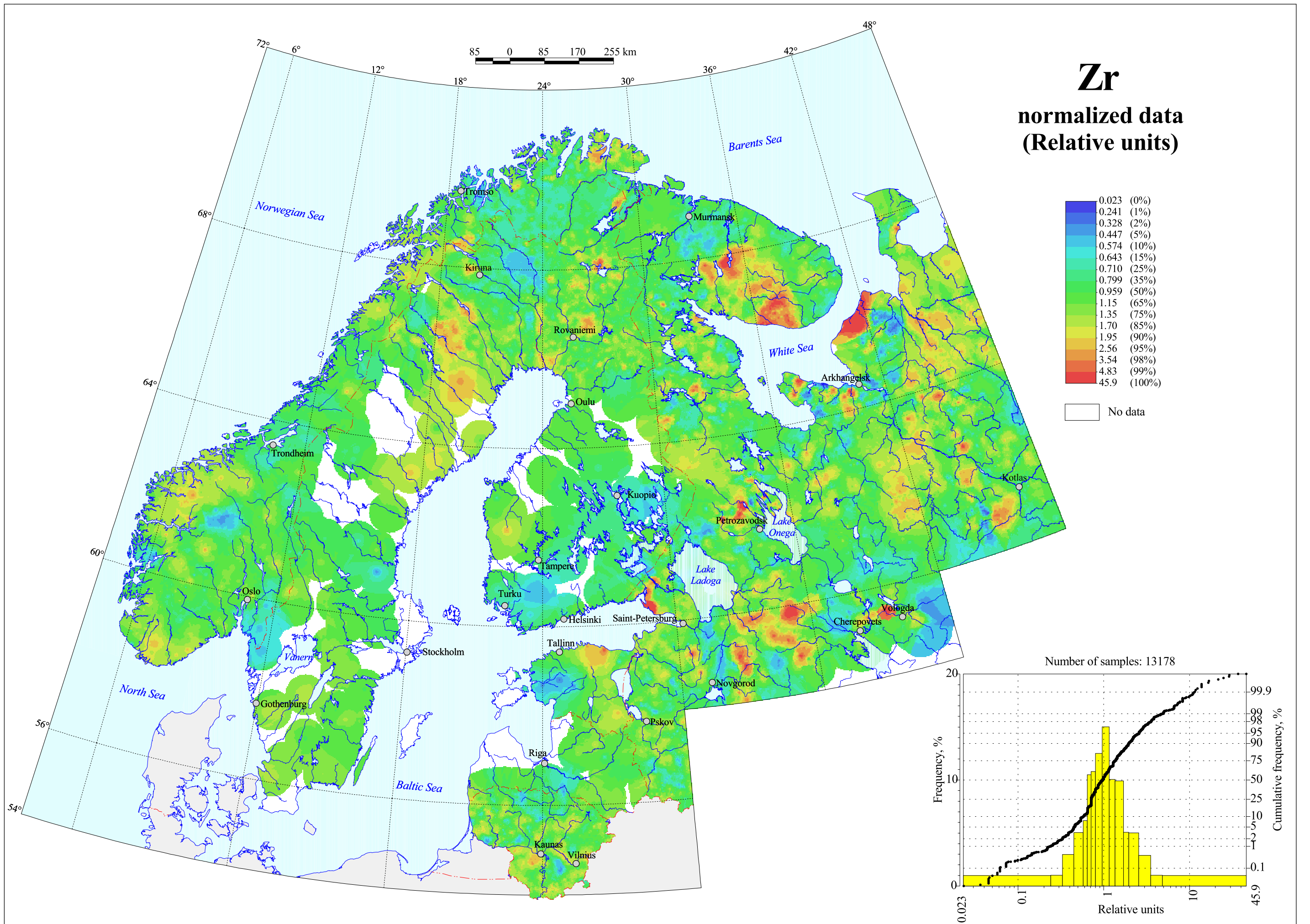
Zirconium in stream sediment
